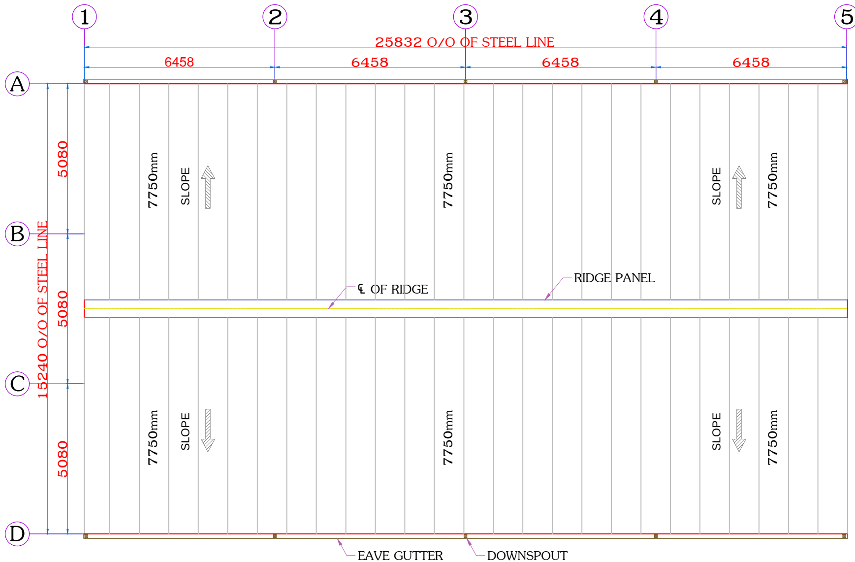
ROOF SHEETING PLAN
